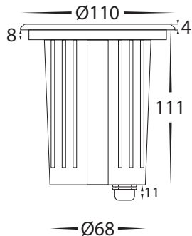
Cutout without Canister Ø98
