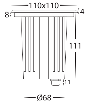
Cutout without Canister Ø98
