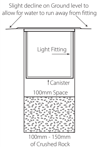
Cutout with Canister Ø104
