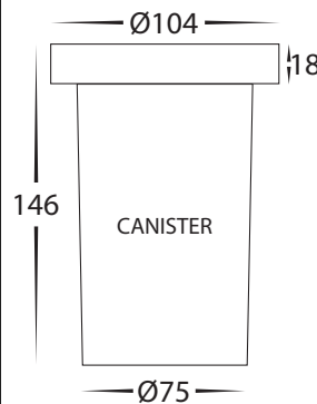
Cutout with Canister Ø104
