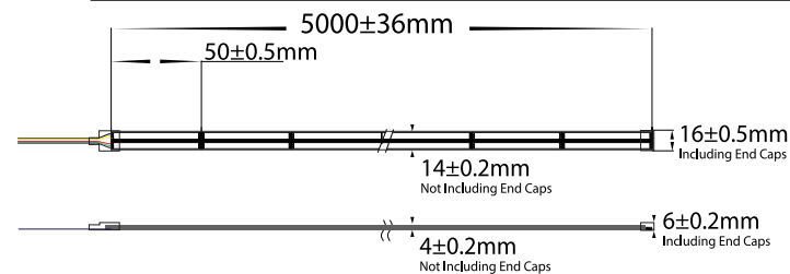
IP67 16mm (W) x 6mm (H) LED Strip Dimensions
