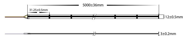
IP54 12mm (W) x 3mm (H) LED Strip Dimensions
