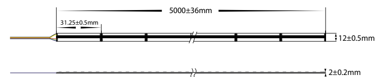
IP20 12mm (W) x 2mm (H) LED Strip Dimensions
