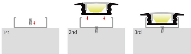
Surface Mounted Installation Method
